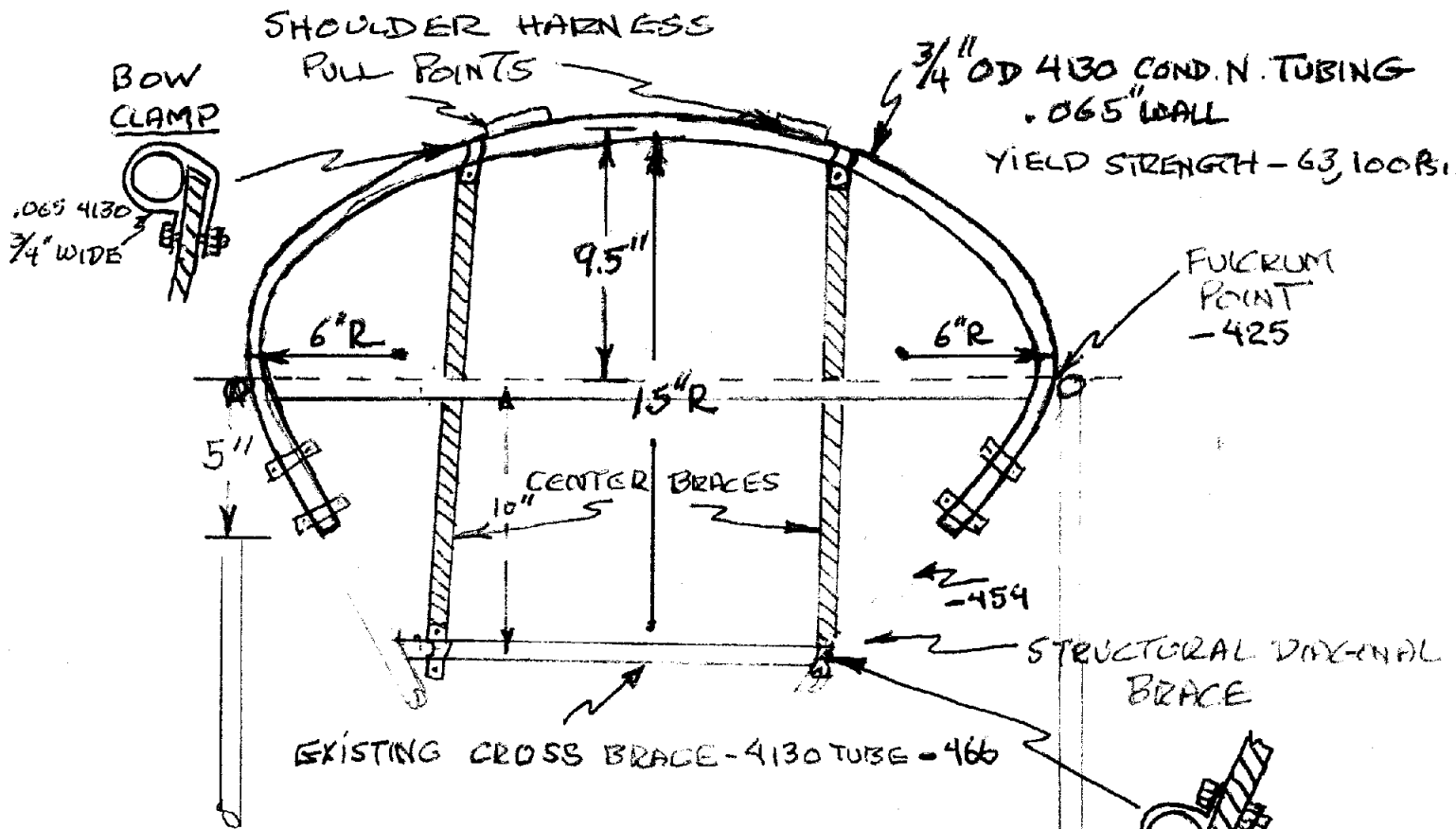
FRONT VIEW (NOT TO SCALE)
